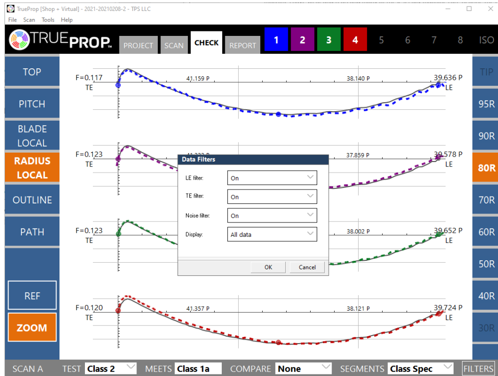
Figure 3 – New 2021 features for automatic detection of blade edges and signal noise filtering.
