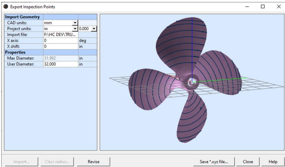
Figure 2 - New debut of the TrueProp Virtual Plug-in for 3D laser scanned propellers.
