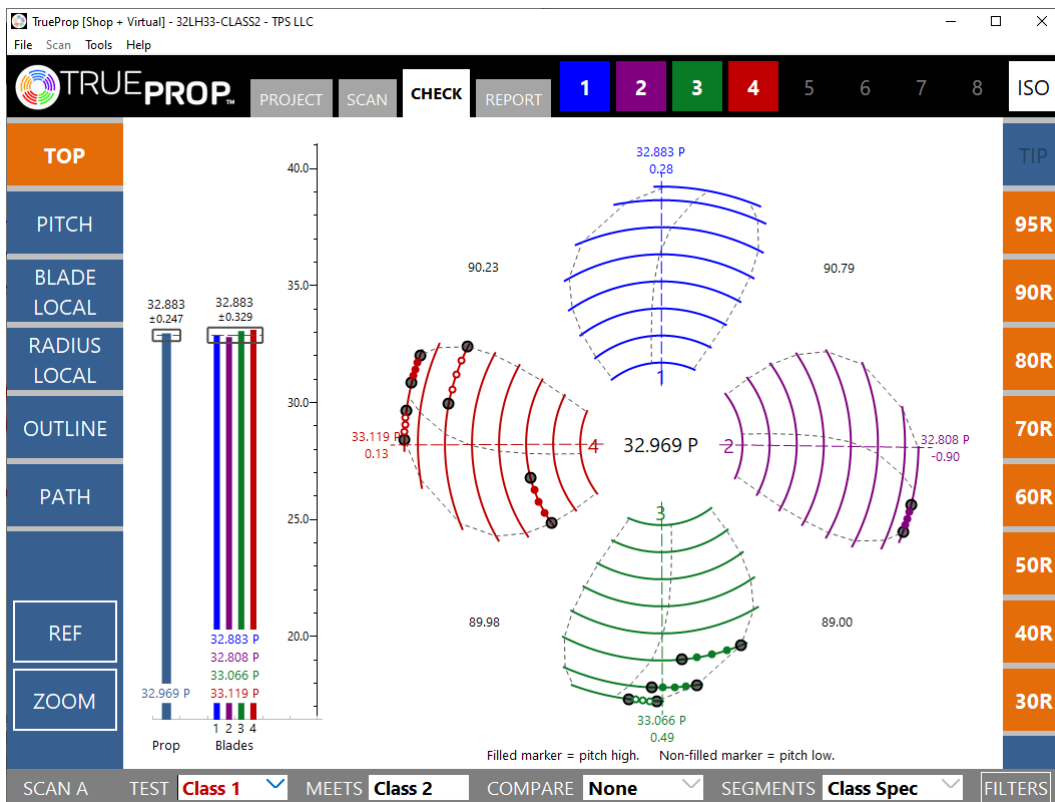
Figure 1 - TrueProp 2021 provides technicians the output they need to inspect and repair propellers.
